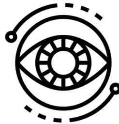
Computer Vision
